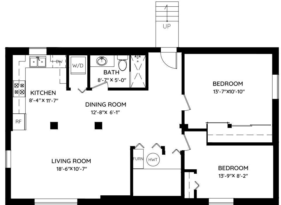
LOWER FLOOR 1,024 SQ.FT. CH: 7'-0"
