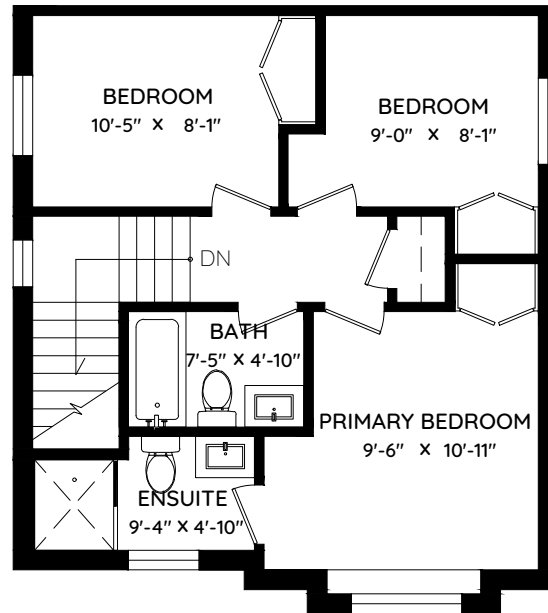
UPPER FLOOR 560 SQ.FT. CH: 9'-0"
