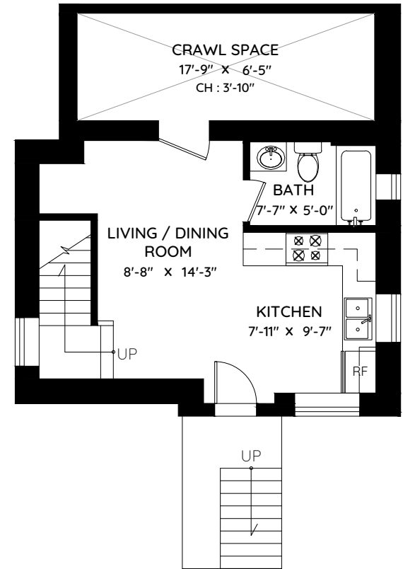
BASEMENT 397 SQ.FT. CH: 8'-0"
