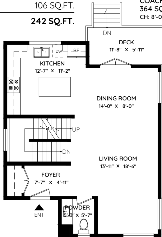
MAIN FLOOR 717 SQ.FT. CH: 9'-0"
