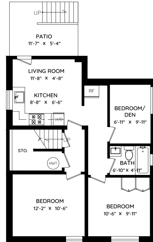
LOWER FLOOR 771 SQ.FT. CH: 8'-0"
