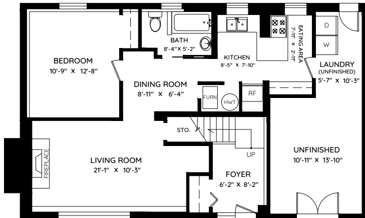
LOWER FLOOR 837 SQ.FT. CH: 7'-4"
