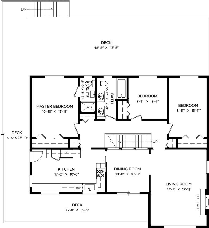
MAIN FLOOR 1,289 SQ.FT. CH: 8'-0"
