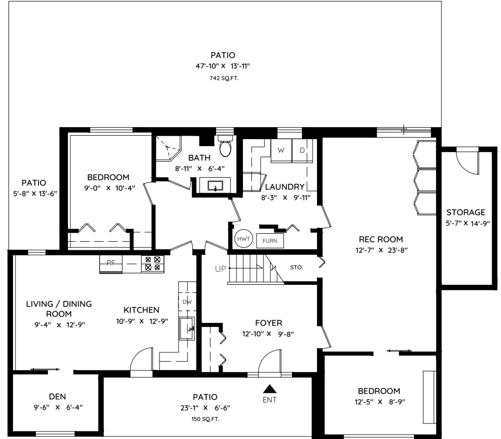
LOWER FLOOR 1,412 SQ.FT. CH: 8'-0"
