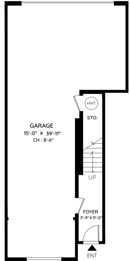
LOWER FLOOR 81 SQ.FT. CH: 8'-0"
