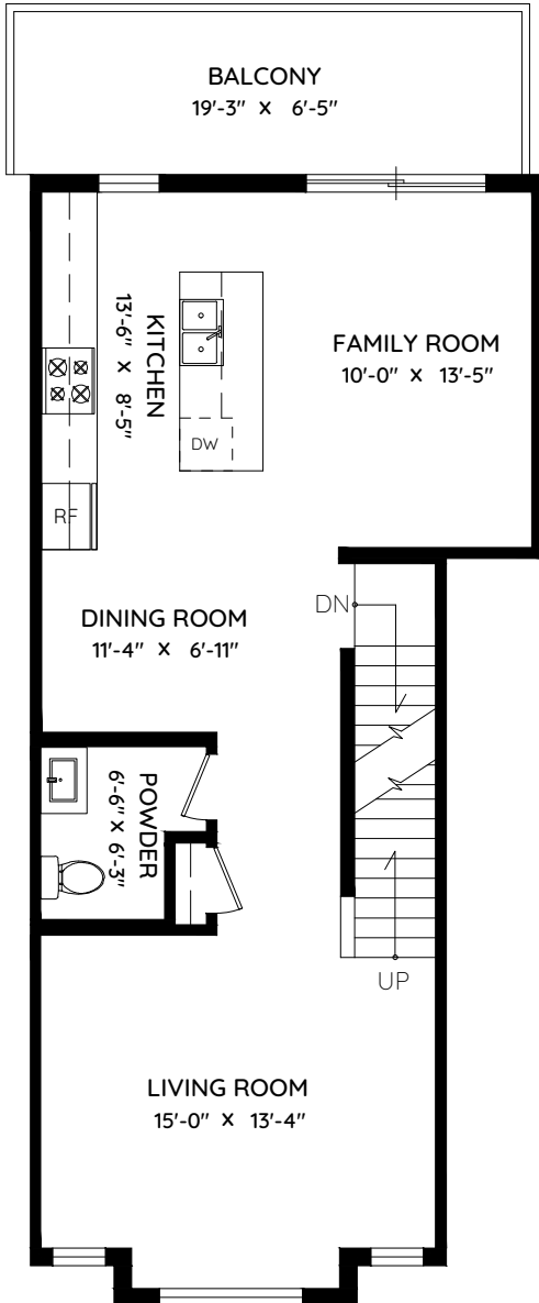
MAIN FLOOR 716 SQ.FT. CH: 8'-11"
