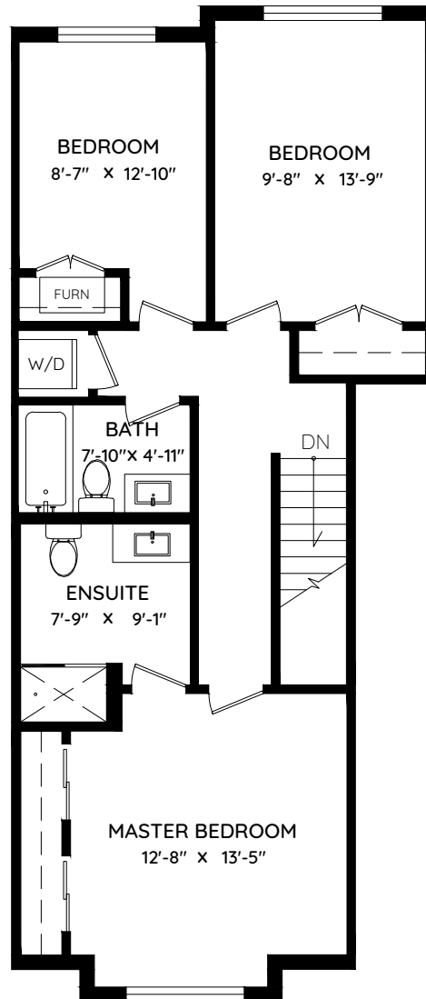
UPPER FLOOR 762 SQ.FT. CH: 8'-0"
