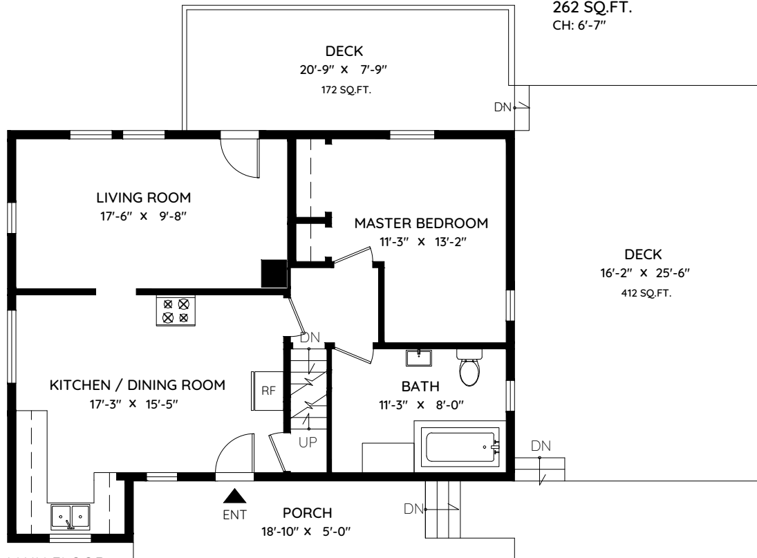
MAIN FLOOR 769 SQ.FT. CH: 8'-4"
