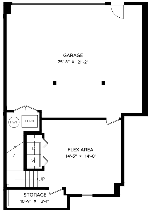
LOWER FLOOR 380 SQ.FT. CH: 7'-8"
