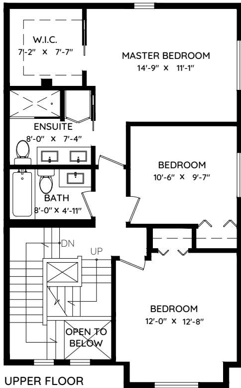
UPPER FLOOR 821 SQ.FT. CH: 8'-0"
